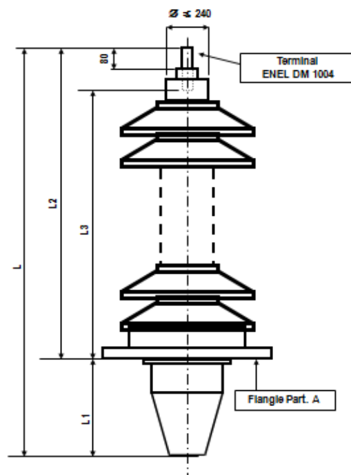
FIGURE 11 – OIL TO AIR BUSHING
