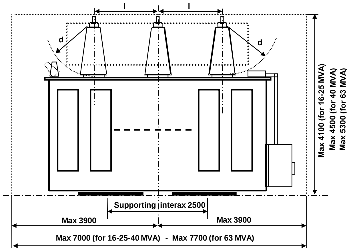
FIGURE 1 – FRONT VIEW OF THE HV SIDE (FOR AIR LINES CONNECTIONS)
