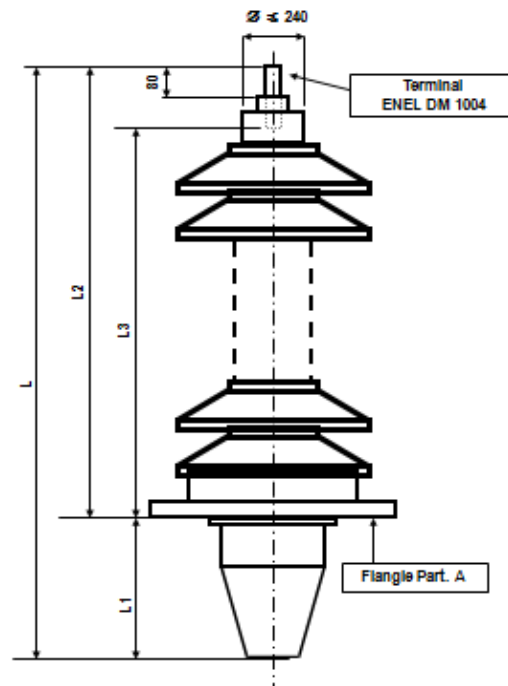
FIGURE 14 – OIL TO AIR BUSHING
