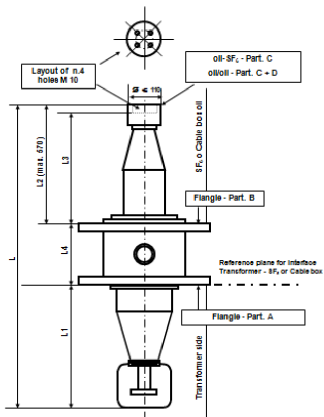
PART B – FLANGE GIS OR CABLE BOX SIDE
