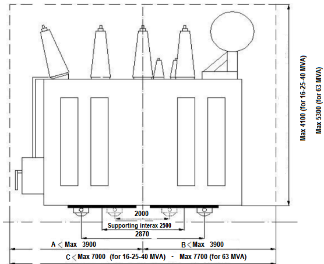
FIGURE 1 – FRONTAL VIEW OF THE HV SIDE (FOR AIR LINES CONNECTIONS)
