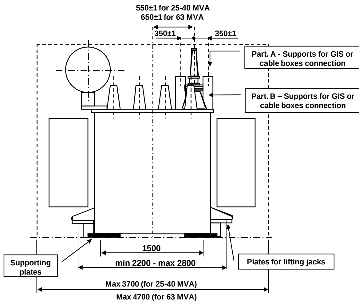
FIGURE 5 – LATERAL VIEW FROM THE MV SIDE FOR GIS CONNECTION OR CABLE TERMINATION BOXES
